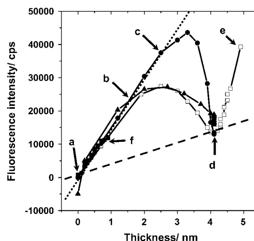
FIGURE 5 Plot of fluorescence intensity versus adsorbed lipid film thickness measured by SPR-SPFS during the vesicle fusion process. Four types of vesicles were compared: POPC ( open squares ); POPC/POPS (4:1) ( solid circles ); POPC/POPS (1:1) ( solid squares ); POPC/DOTAP (4:1) ( solid triangles ). The arrows indicate ( a ) before the addition of vesicles, ( b ) initial linear phase (adsorption of vesicles), ( c ) onset of vesicle rupture (for POPC/POPS (4:1)), ( d ) complete coverage with planar bilayer, and ( e ) additional adsorption of vesicles (for POPC), respectively. The sign ( f ) indicates the profile of POPC/POPS (1:1). The dotted and dashed lines were given to indicate the linearity of fluorescence intensity versus film thickness for adsorbed vesicles and planar bilayers, respectively.
