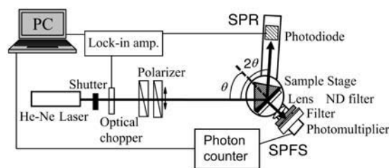
FIGURE 2 Schematic diagram of the SPR-SPFS setup.
